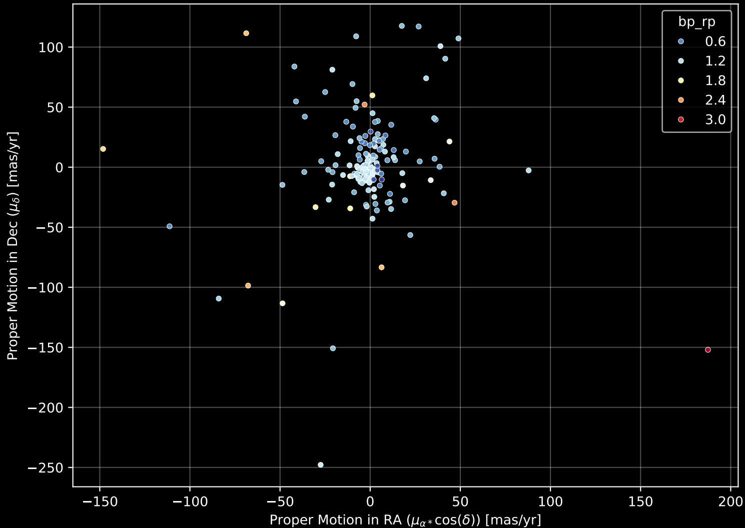
APOGEE DR17 Field: [CVZTILE_093+27_btx] Proper Motion Diagram (n= 181)
