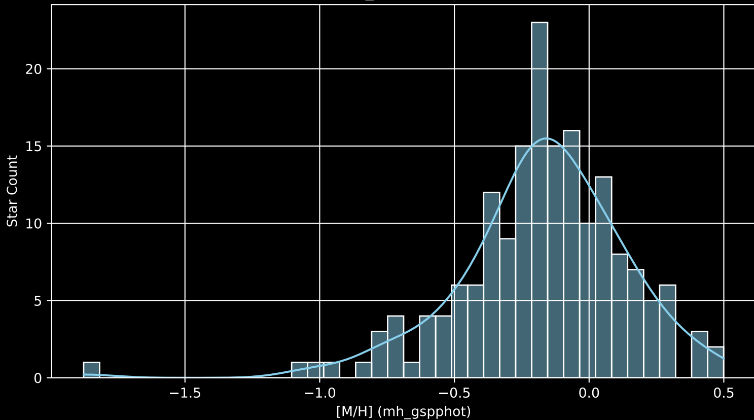
APOGEE DR17 Field: [CVZTILE_093+27_btx [M/H] (mh_gspphot) (n= 177)
