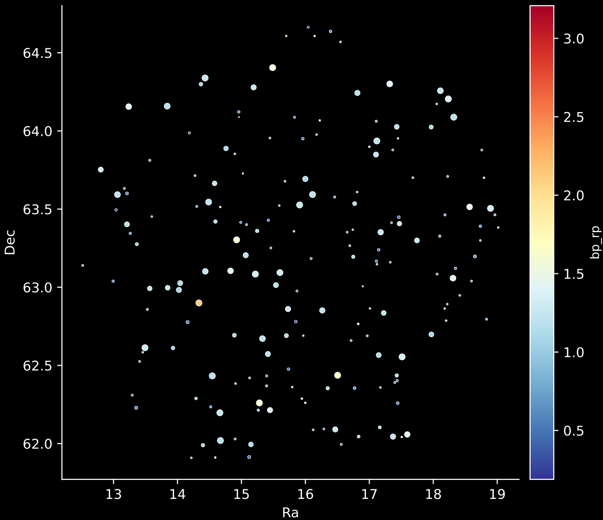
APOGEE DR17 Field: [CVZTILE_093+27_btx] Stars: 181
