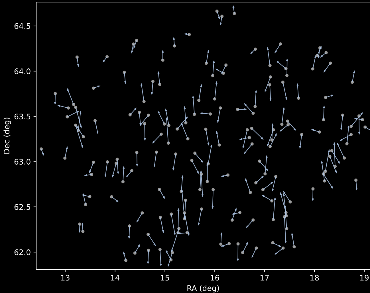
APOGEE DR17 Cluster 1 Proper Motion Vectors (n=163)
