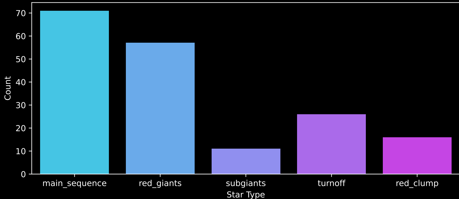
APOGEE DR17 Field: [CVZTILE_093+27_btx] Count plot of Star Type
