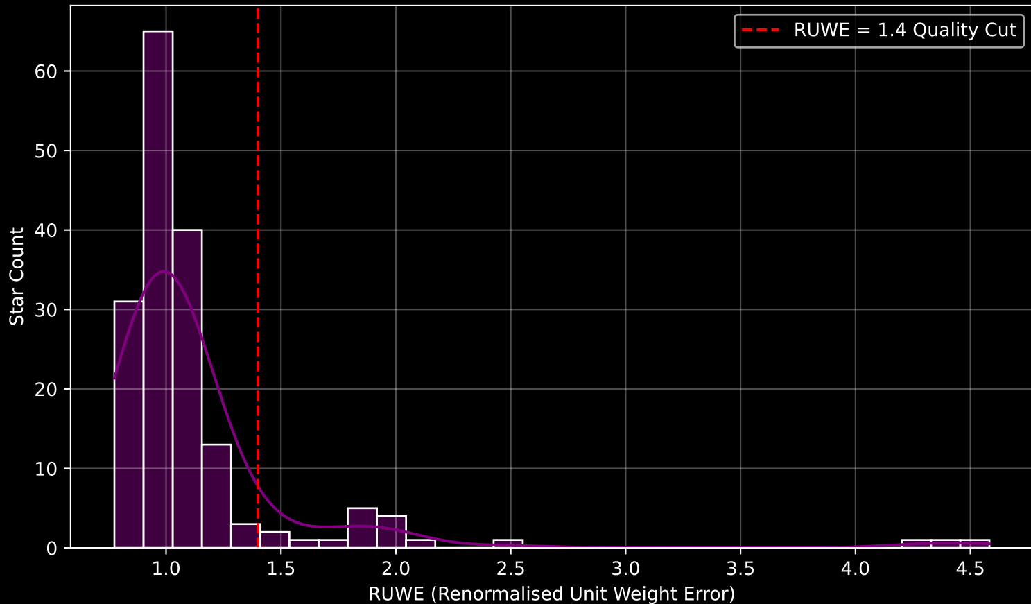
GAPOGEE DR17 Field [CVZTILE_093+27_btx] RUWE Distribution (n= 170)
