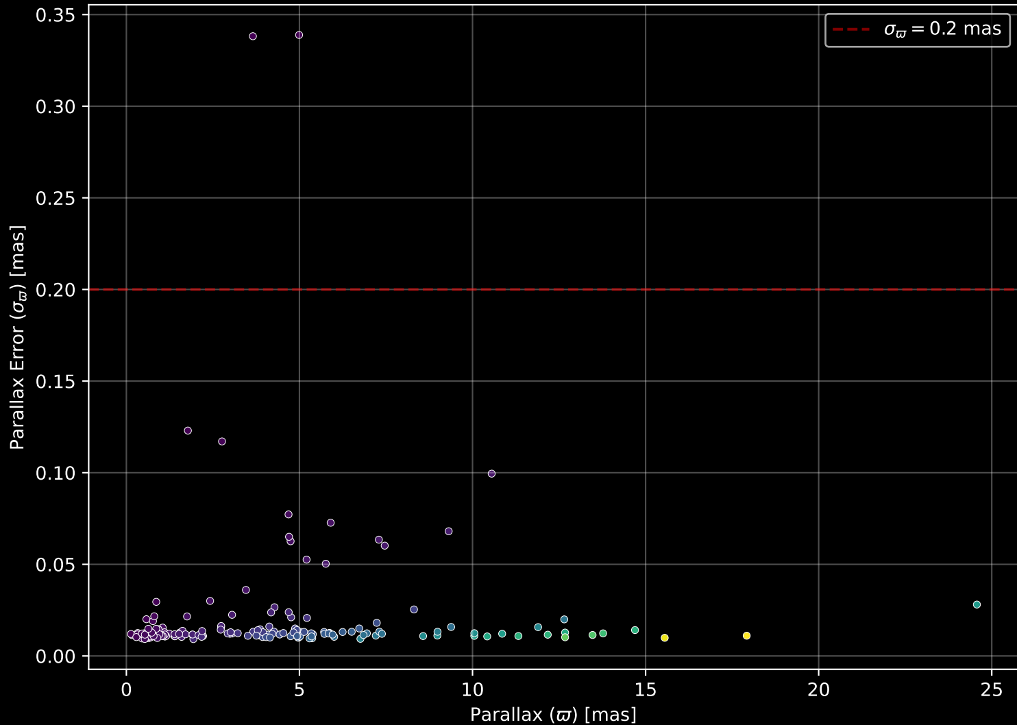
APOGEE DR17 Field: [CVZTILE_093+27_btx] Parallax Quality (n= 181)
