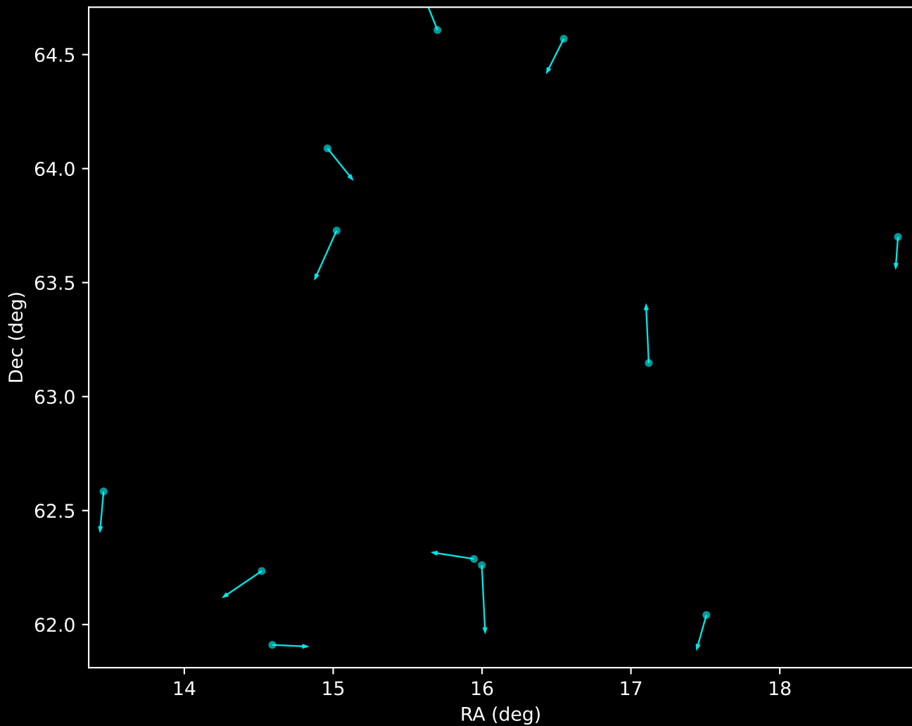
APOGEE DR17 Noise Stream Proper Motion Vectors (n=12)
